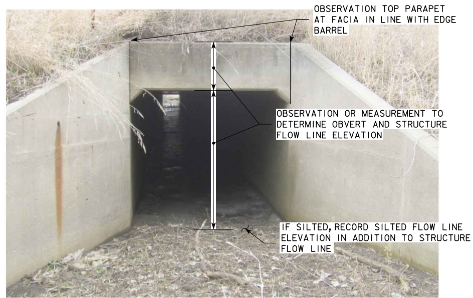
SINGLE BOX CULVERT
