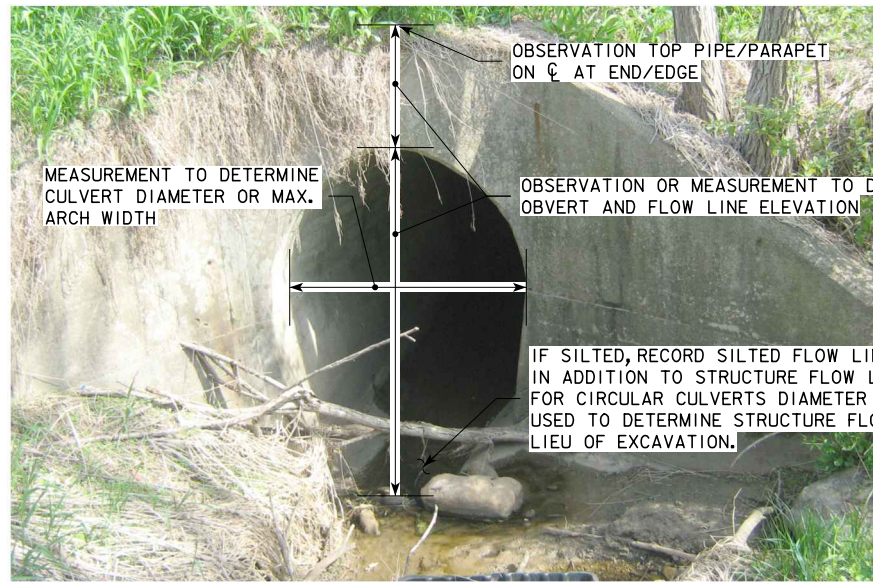
CIRCULAR / ARCH CULVERTS
