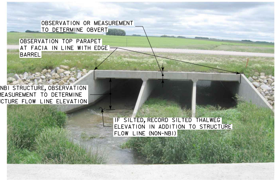
DOUBLE OR TRIPLE BOX CULVERT
