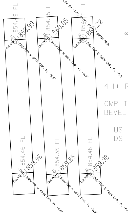
EXAMPLE SYMBOLOGY SURVEY CAD FILE
