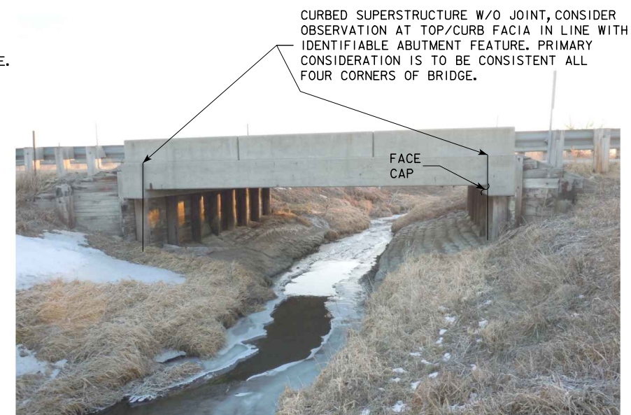
CURB W/ INTEGRAL SUPERSTRUCTURE
