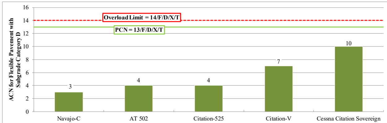
Figure 1. ACN–PCN comparison for Runway 16/34.
