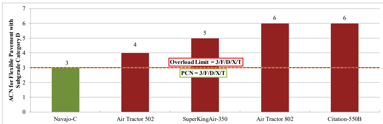
Figure 2. ACN–PCN comparison for Runway 16-34.
