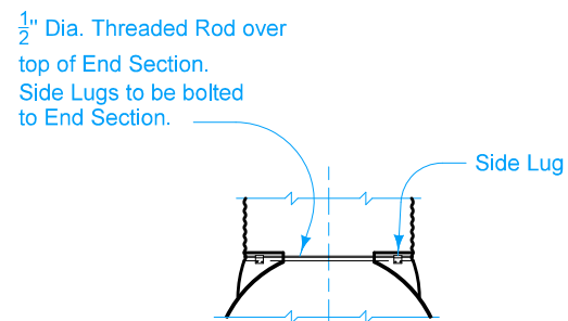
CONNECTOR (30"-60" Dia.)
