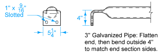
PARALLEL SAFETY BARS
