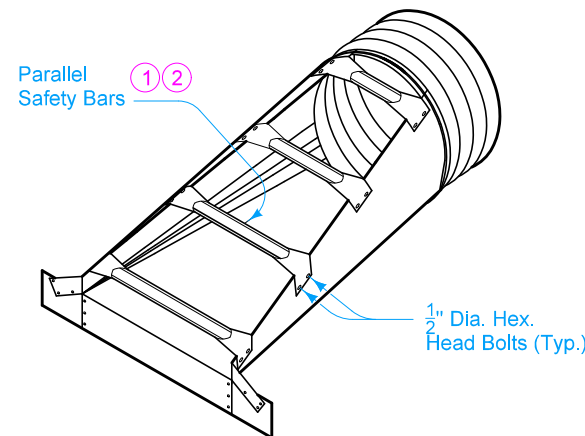
PERSPECTIVE VIEW OF APRON
