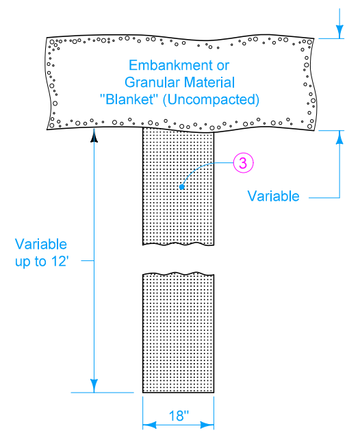
TYPE 3 INSTALLATION TRENCH DRAIN SECTION C-C
