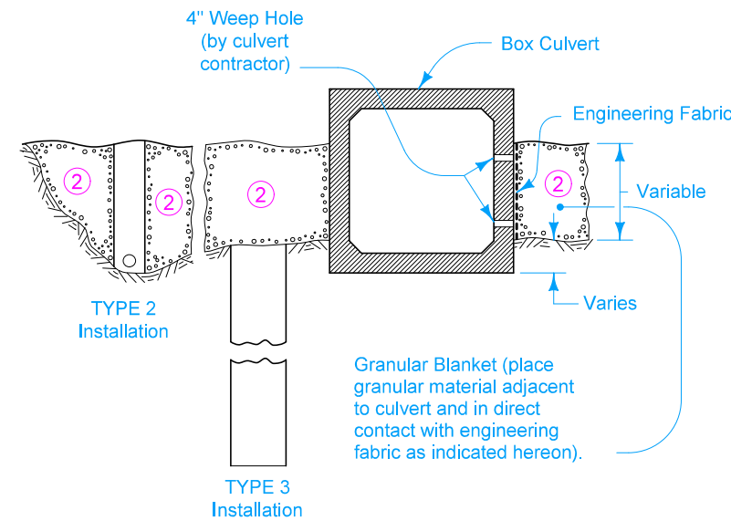
SECTION E-E SUBSOIL DRAINAGE
