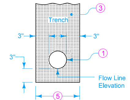
TUBING PLACEMENT DETAIL ALL TYPES
