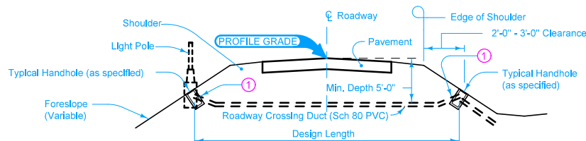
TYPICAL SECTION WHERE FORESLOPES ARE STEEPER THAN 6:1
