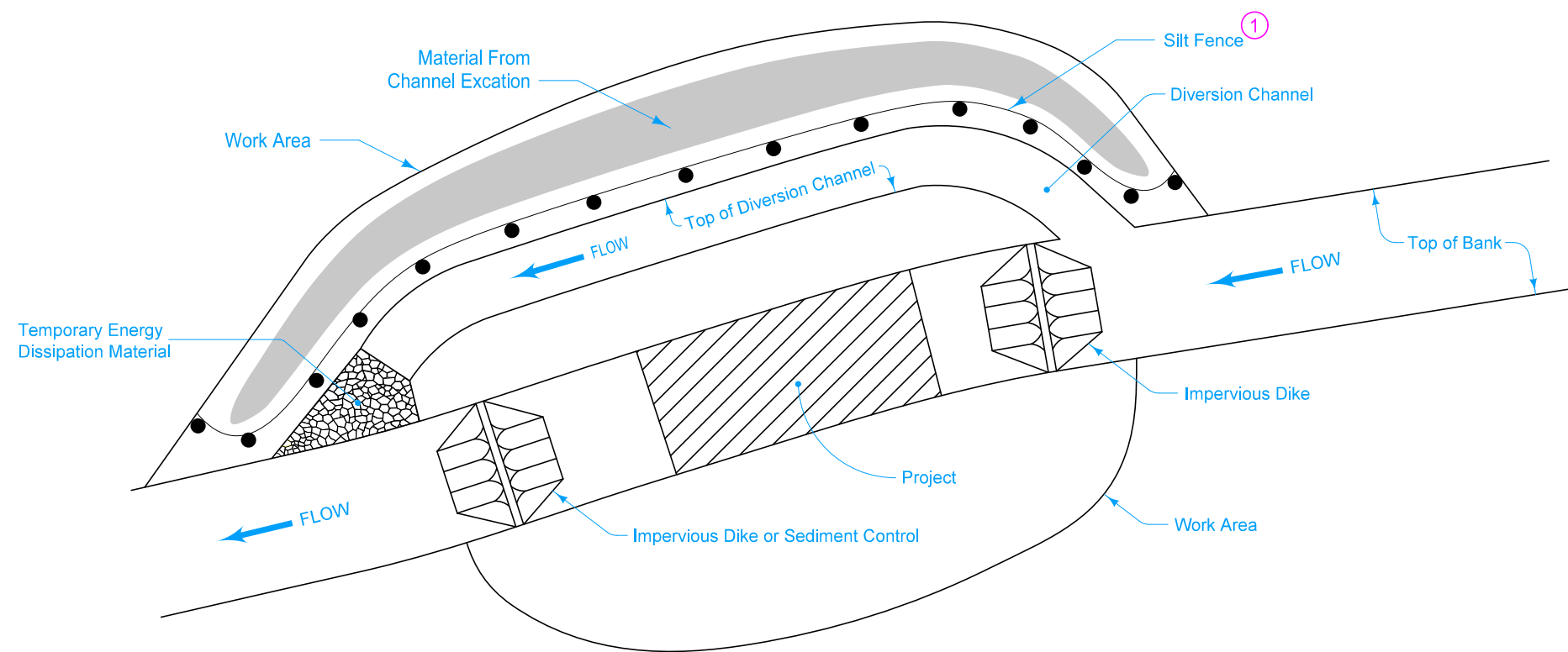
DIVERSION CHANNEL
