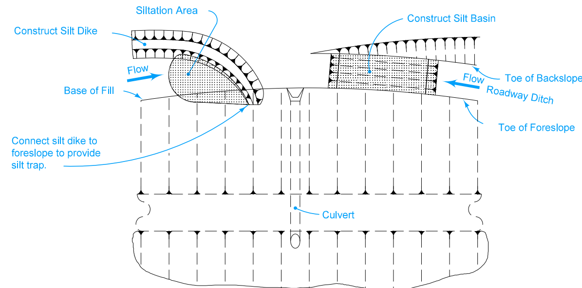
TYPICAL PLAN WITH PERMANENT CULVERT INSTALLATION
