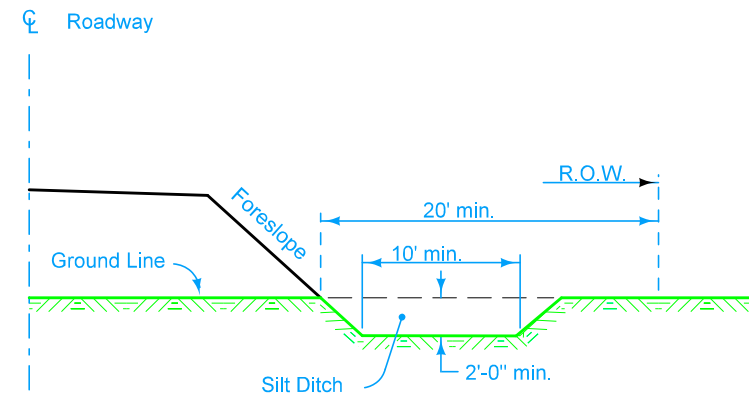
SILT DITCH
