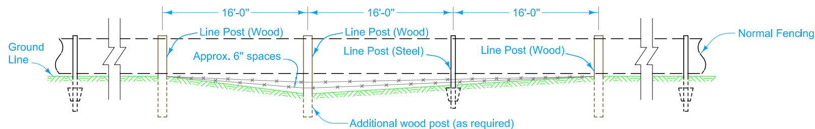
LINE FENCE AT MINOR GROUND DEPRESSIONS
