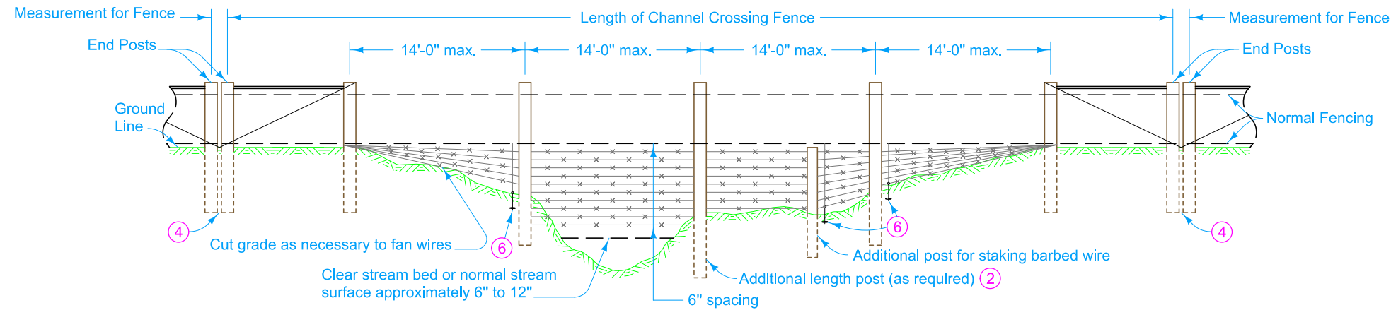
CHANNEL CROSSING FENCE - TYPE "A"
