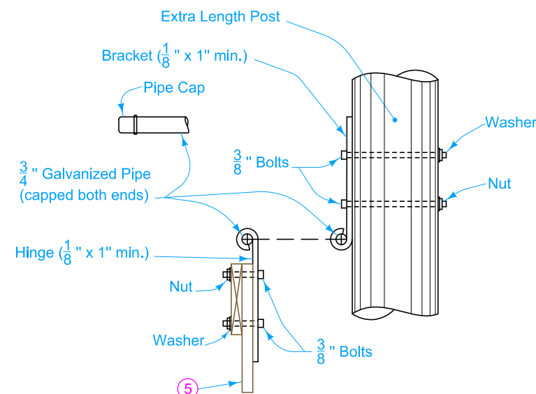
FLOODGATE HINGE AND BRACKET
