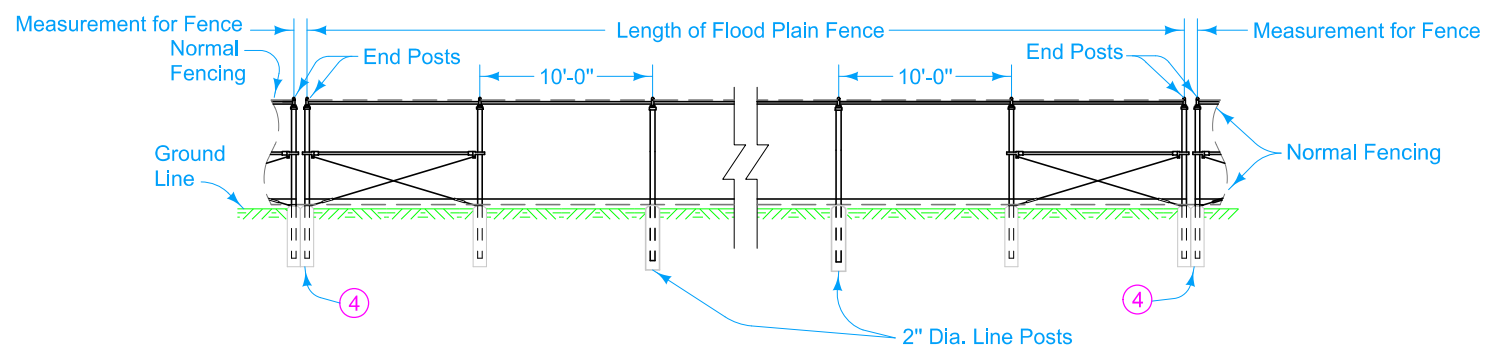
FLOOD PLAIN FENCE
