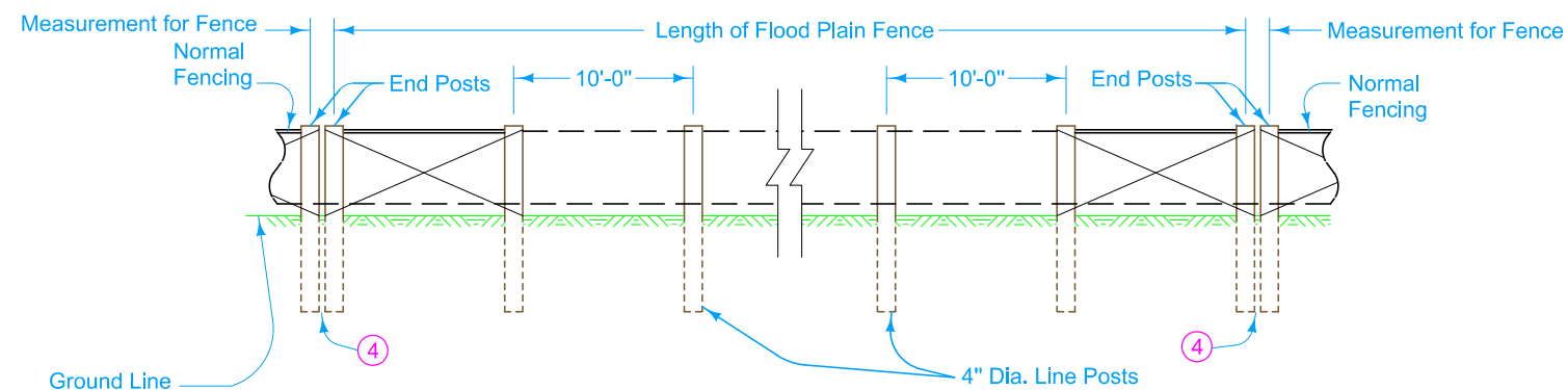
FLOOD PLAIN FENCE
