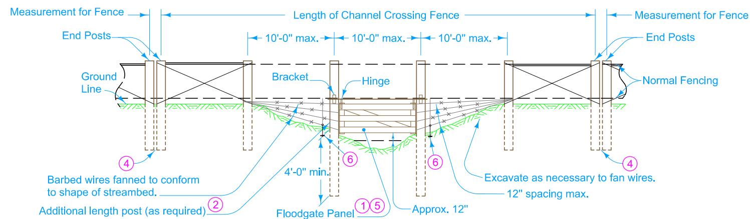
CHANNEL CROSSING FENCE - TYPE "B"
