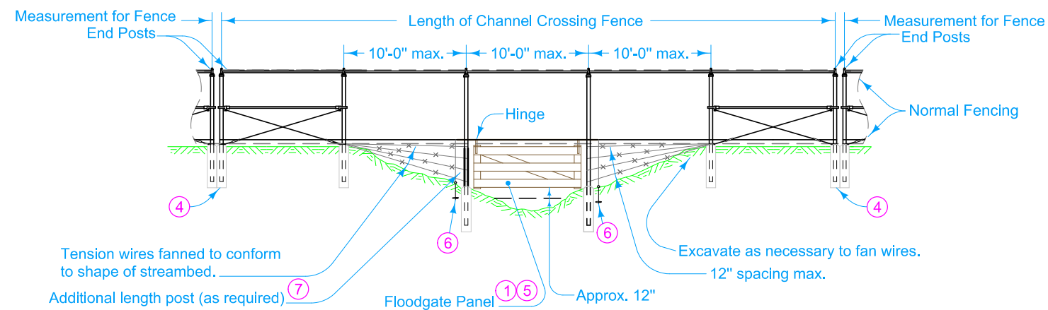
CHANNEL CROSSING FENCE - TYPE "B"
