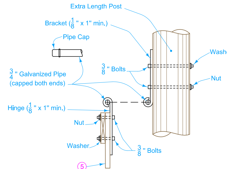
FLOODGATE HINGE AND BRACKET
