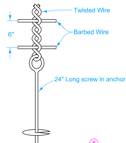
BARBED WIRE ANCHOR
