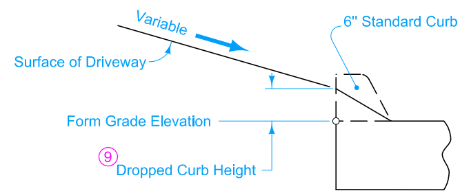
SECTION C-C (Standard Curb)
