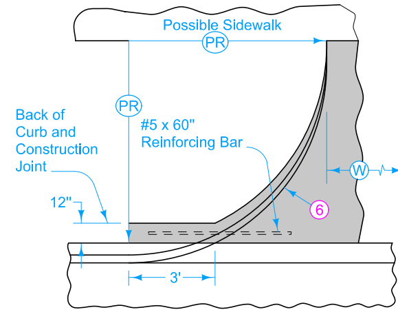
DETAIL 'A' CASE 1 ENTRANCE
