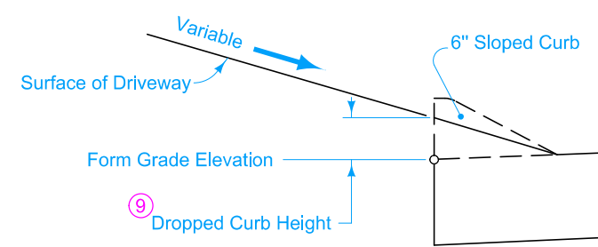
SECTION C-C (Sloped Curb)
