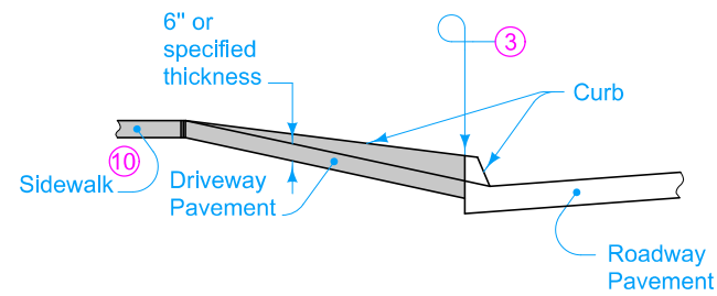
SECTION B-B (Cases 2 Entrance)
