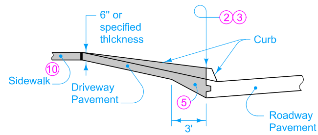
SECTION A-A (Case 1 Entrance)
