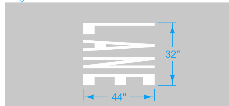
LANW LANE WORD MARKING (White)
