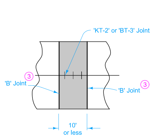
FULL ROADWAY WIDTH PATCH
