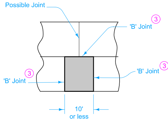
ONE LANE WIDTH PATCH
