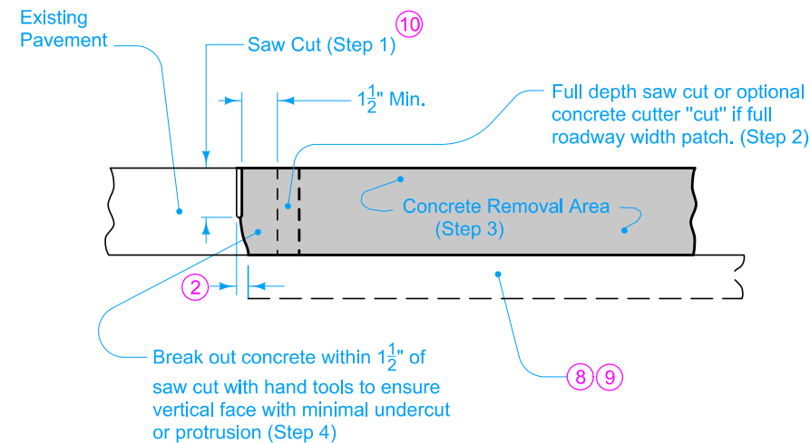
PAVEMENT REMOVAL
