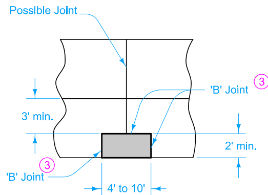
PARTIAL LANE WIDTH PATCH
