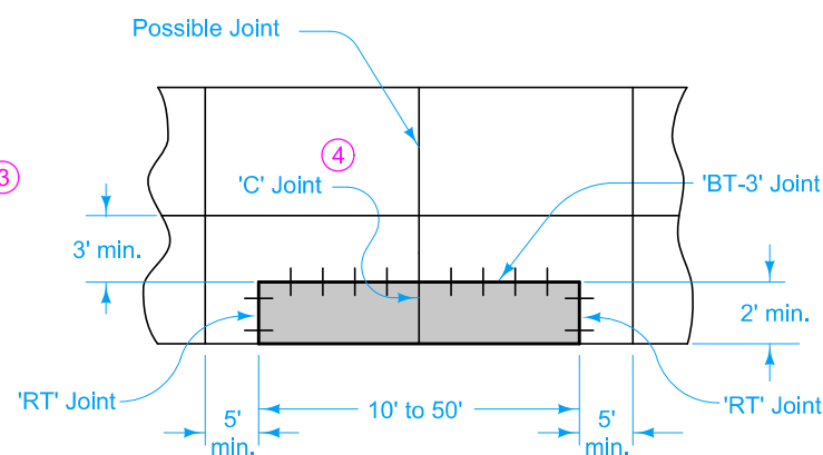
PARTIAL LANE WIDTH PATCH
