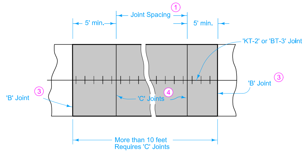
FULL ROADWAY WIDTH PATCH
