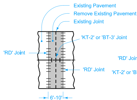
FULL ROADWAY WIDTH PATCH
