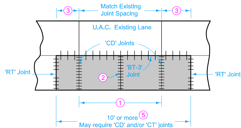
ONE LANE WIDTH PATCH
