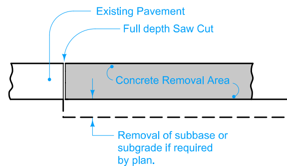
PAVEMENT REMOVAL DETAILS
