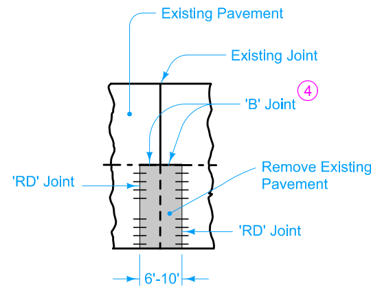
ONE LANE WIDTH PATCH
