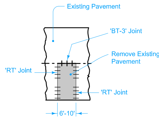
ONE LANE PATCH (NO OPPOSING JOINT)
