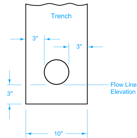
DRAIN PLACEMENT
