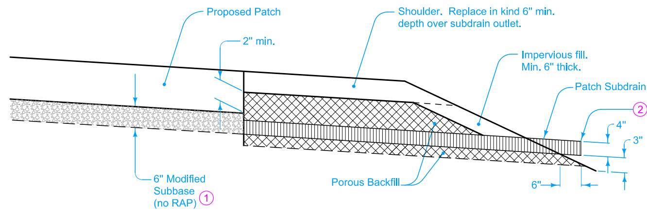
MODIFIED SUBBASE AND SUBDRAIN WITHOUT LONGITUDINAL SUBDRAIN
