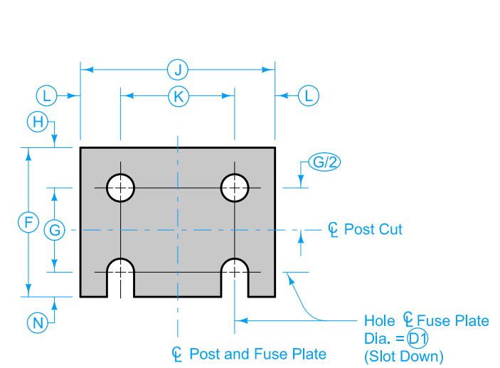
FUSE PLATE (Thickness T_3 )
