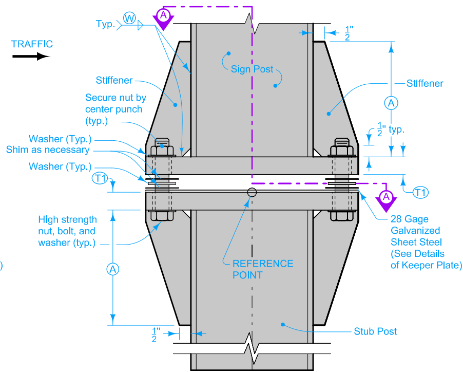
BREAKAWAY BASE Side View (Alternate 2)
