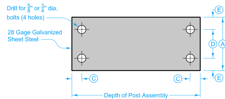
KEEPER PLATE
