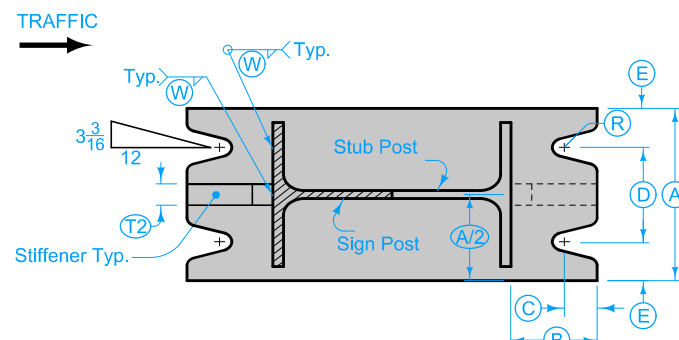
SECTION A-A PLAN - BASE (ALTERNATE 2)
