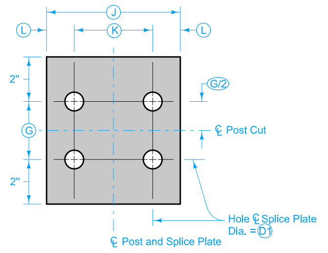
SPLICE PLATE (Thickness T_4 )
