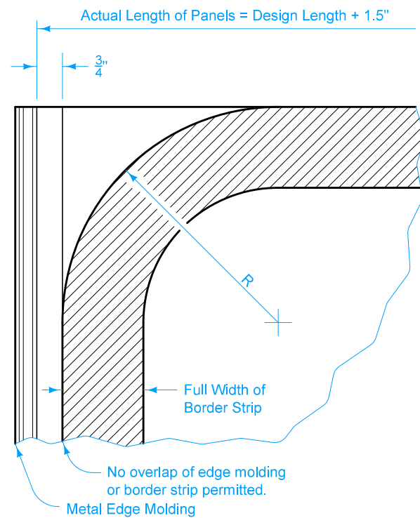
EDGE MOLDING BORDER STRIP DETAIL
