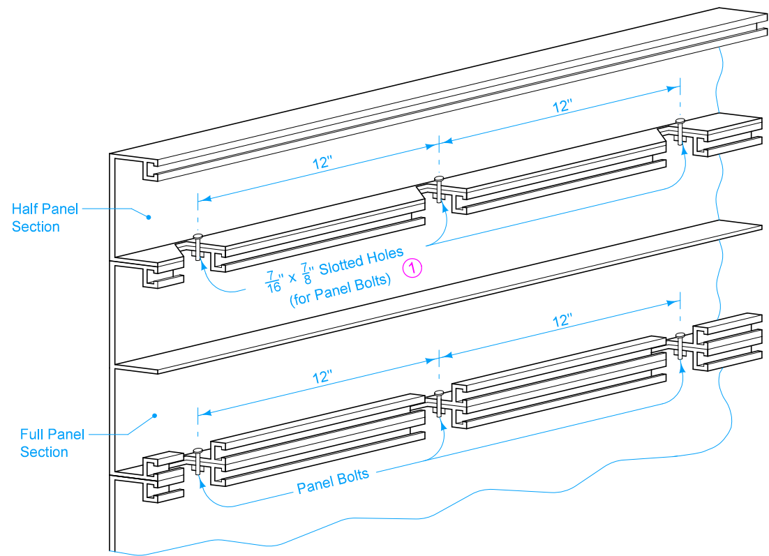
ASSEMBLY DETAIL
