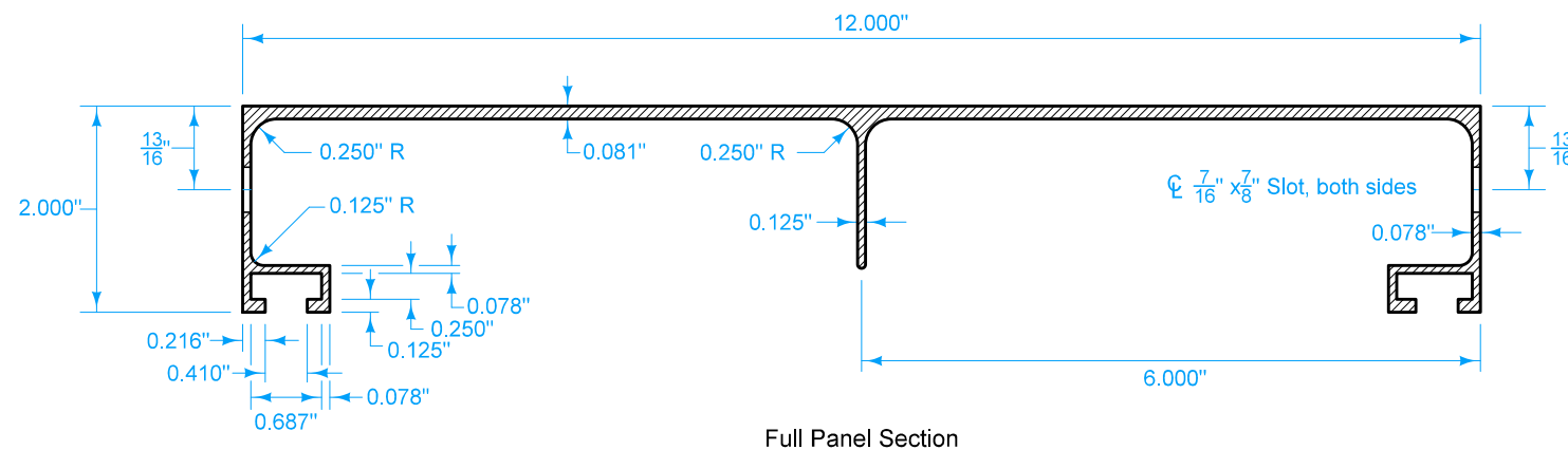
STANDARD STRUCTURAL SIGN PANELS
