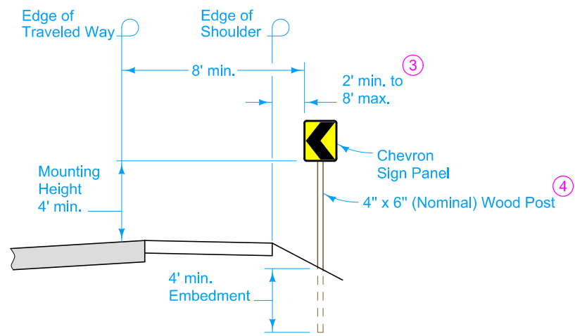
TYPICAL SECTION
