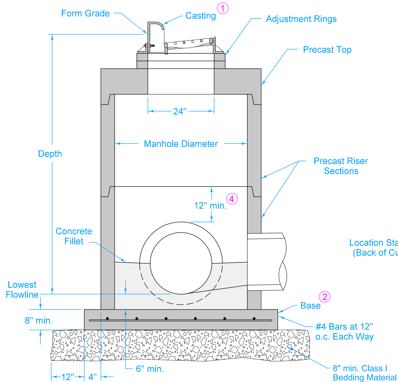
TYPICAL SECTION
