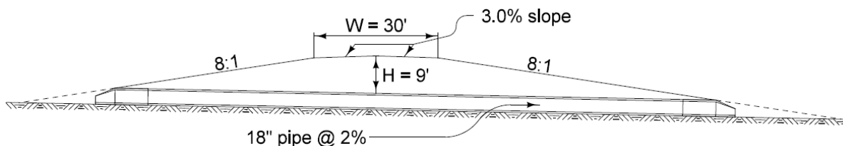
Figure 2: Cross section of entrance for Example 1.
