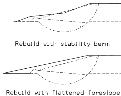
Figure 6: Slope repairs using geometric components (from Lohnes, et. al., 2001).
