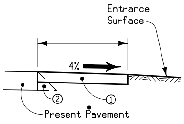
Section A-A Without Fillet
