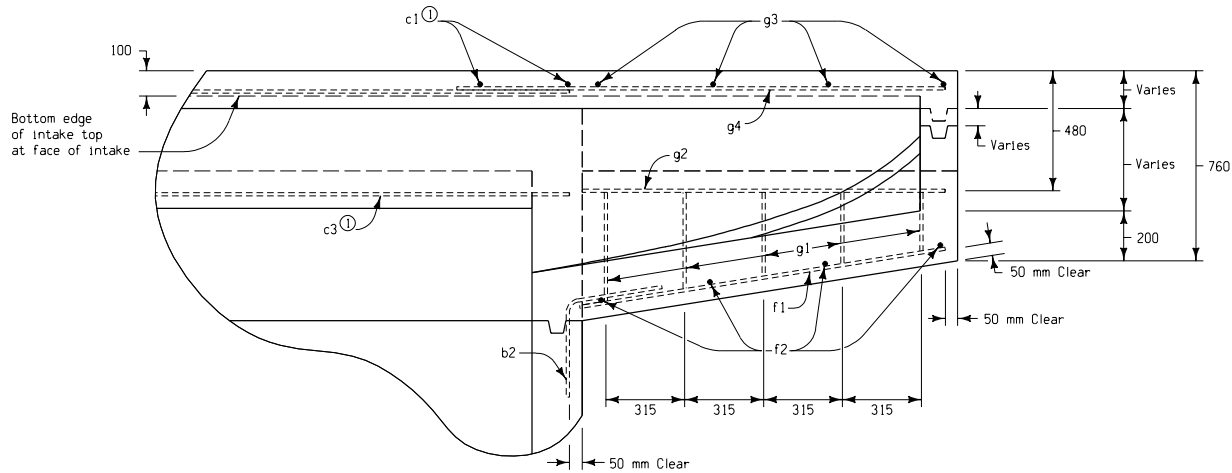
SECTION E-E
