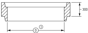
SECTION E-E
