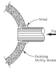
PLAN VIEW CONNECTION TO CIRCULAR UTILITY ACCESS
