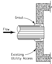
PLAN VIEW CONNECTION TO RECTANGULAR UTILITY ACCESS
