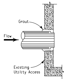
ELEVATION VIEW CONNECTION TO RECTANGULAR UTILITY ACCESS
