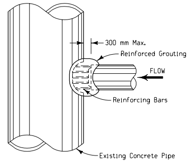
TEE CONNECTION
