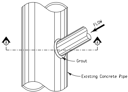
WYE CONNECTION
