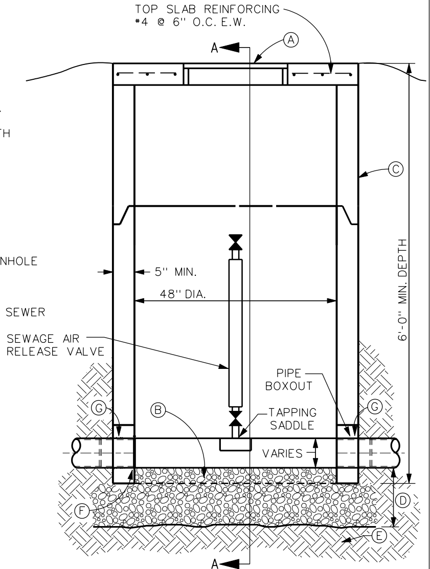
HALF SECTION SECTION A-A
