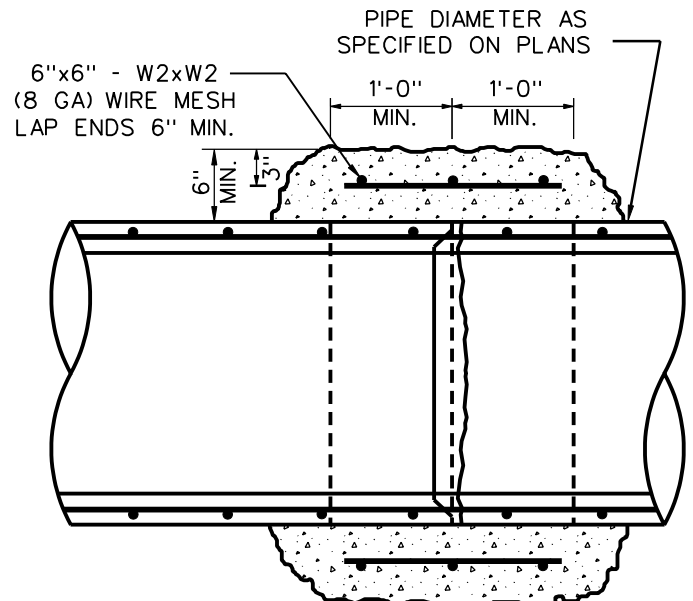
DETAIL OF TYPE II CONCRETE COLLAR CONNECTION
