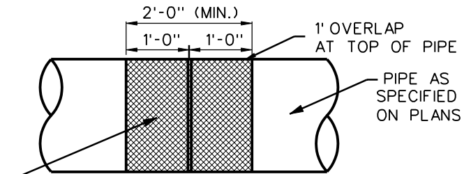
PIPE JOINT WRAPPING (ONLY WHERE SPECIFIED)
