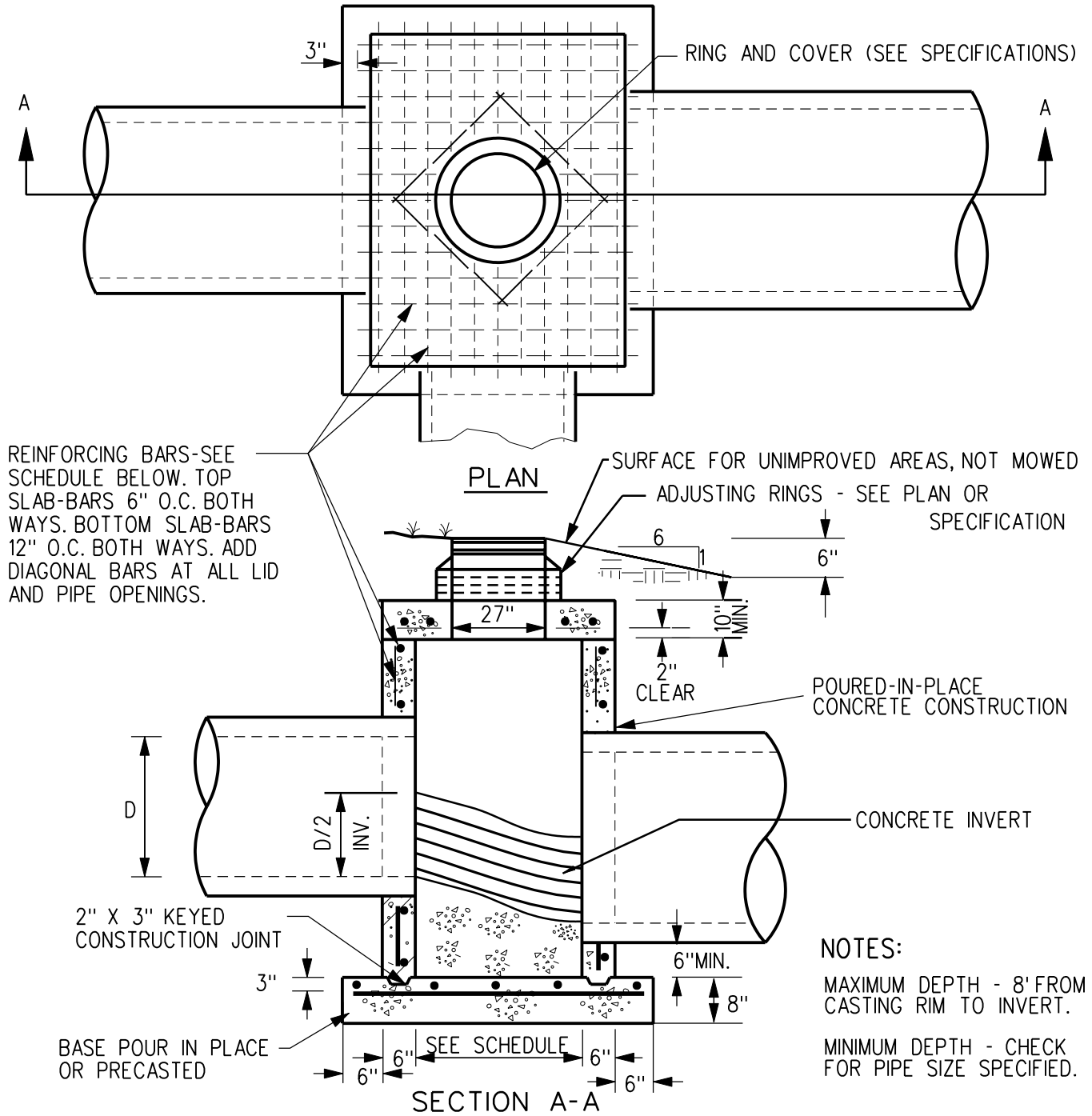
MIN. MANHOLE SIZE AND STEEL SCHEDULE
