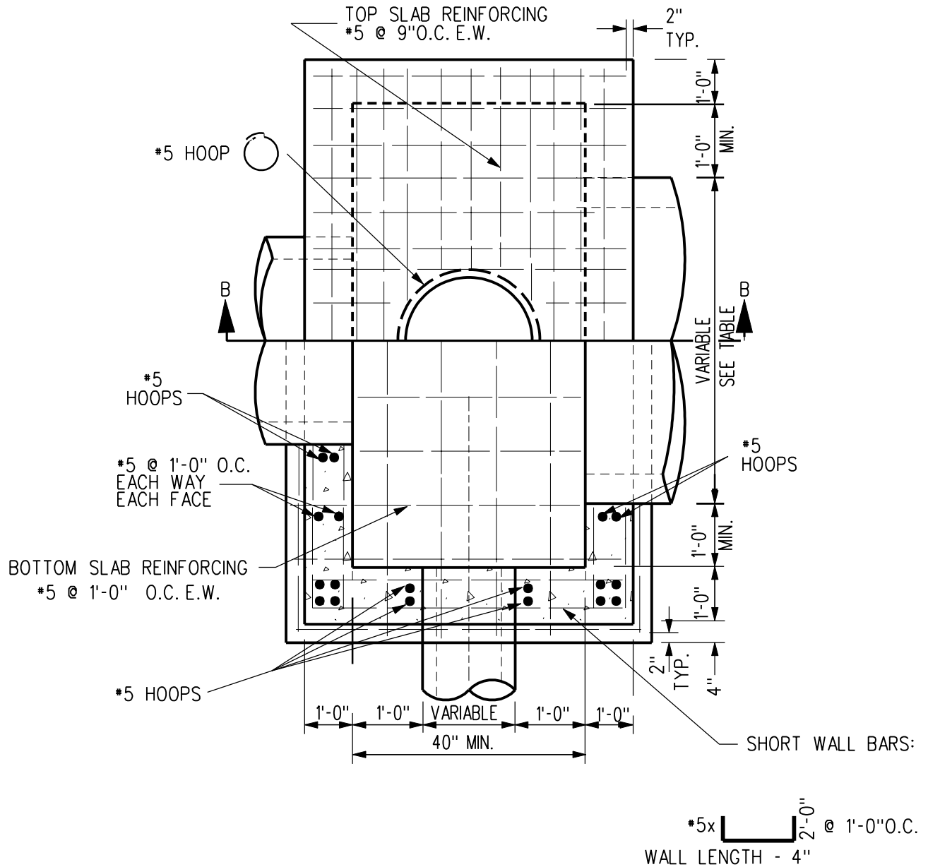
PLAN
