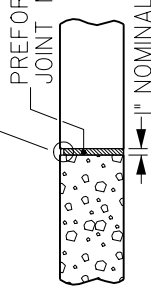
'E' JOINT
