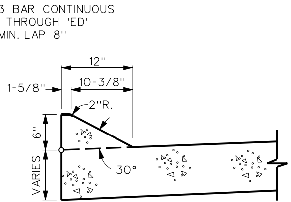
INTEGRAL 6" SLOPED CURB
