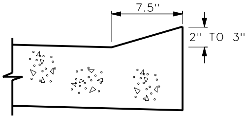
DRIVEWAY DROP CURB
