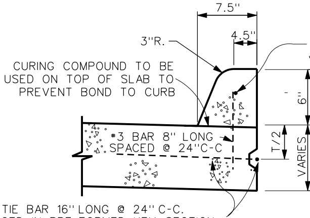
REMOVABLE PCC CURB
