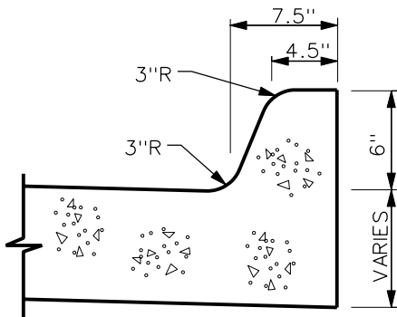
6" PCC INTEGRAL CURB
