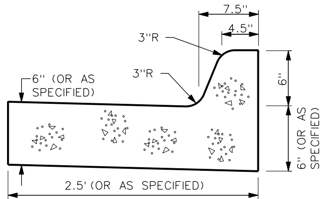
STANDARD PCC CURB & GUTTER*
