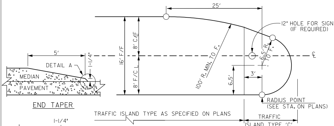
TRAFFIC ISLAND NOSE TYPE II
