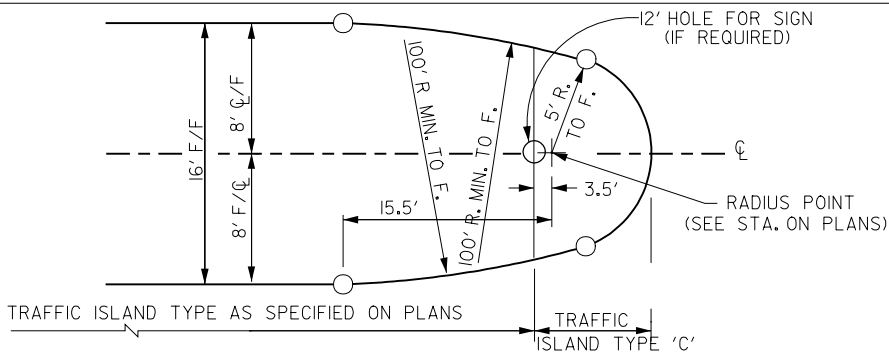
TRAFFIC ISLAND NOSE TYPE I
