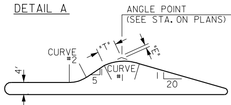
TRAFFIC ISLAND CURVE DETAILS
