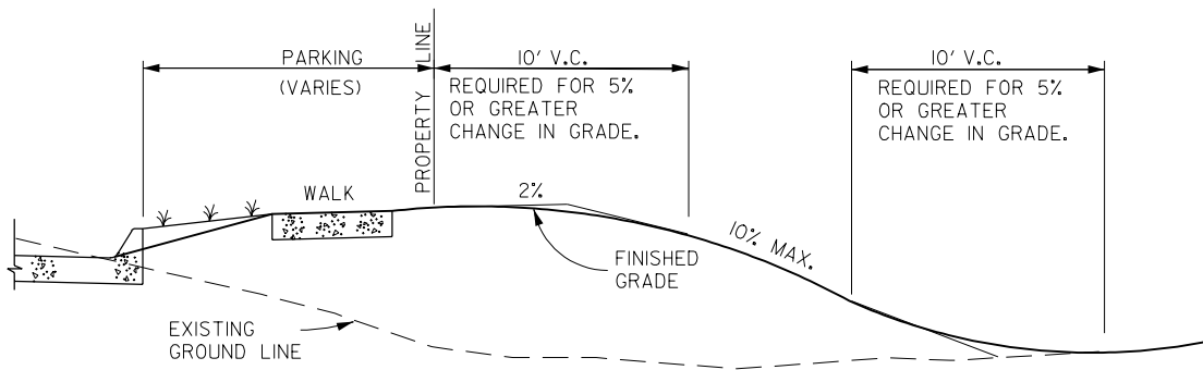
DRIVEWAY GRADING DETAIL IN FILL SECTION (Q PROFILE SHOWN)
