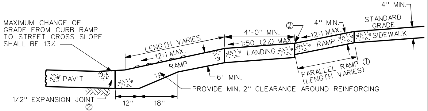
SECTION A-A SIDEWALK AND CURB DROP FOR NEW PAVING
