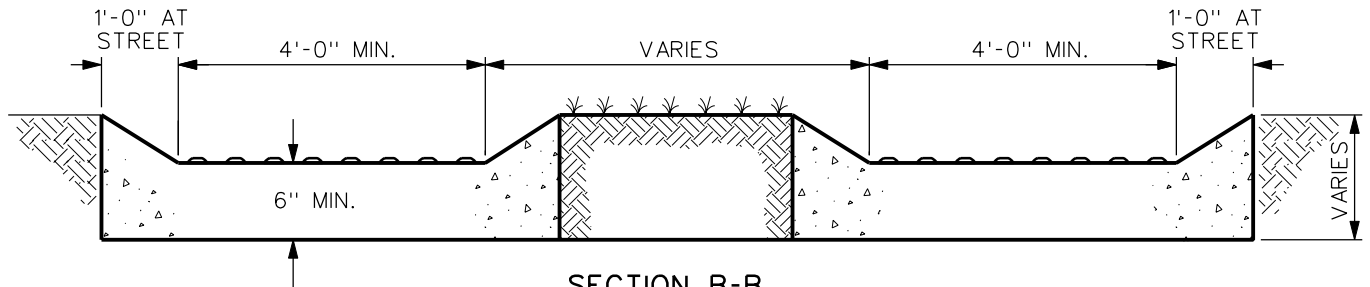
SECTION B-B
