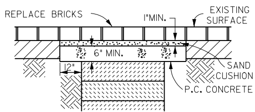
BRICK PAVEMENT
