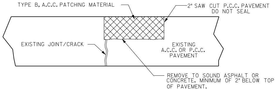
PARTIAL DEPTH A.C.C. PATCH
