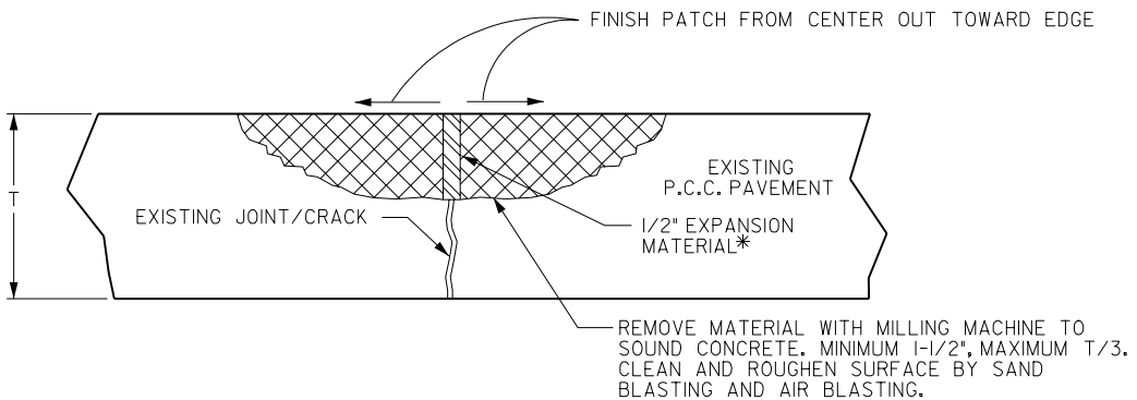
TYPE B PARTIAL DEPTH P.C.C. PATCH
