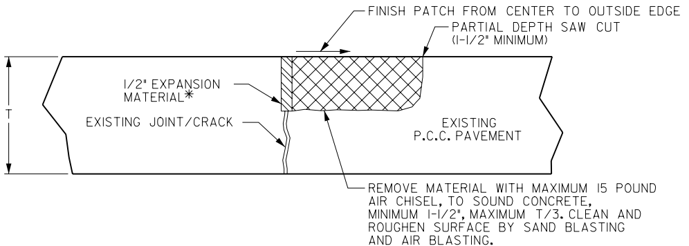
TYPE A PARTIAL DEPTH P.C.C. PATCH
