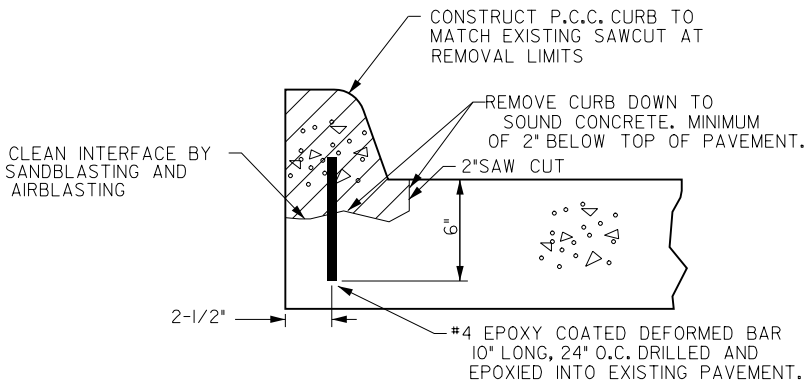
CURB REPLACEMENT - PARTIAL DEPTH
