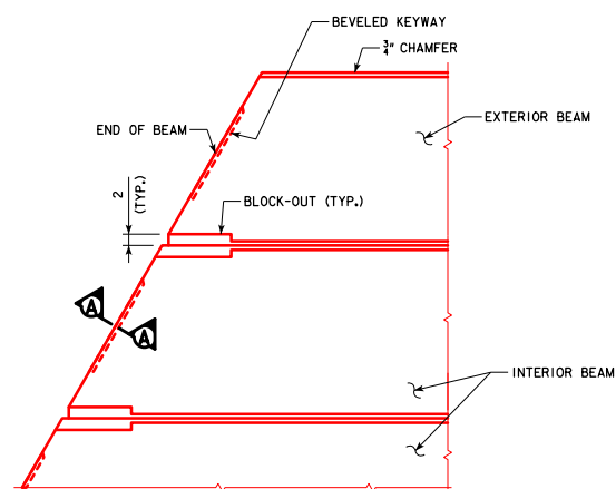
PARTIAL PLAN (30° SKEW SHOWN, 15° SKEW SIMILAR)
