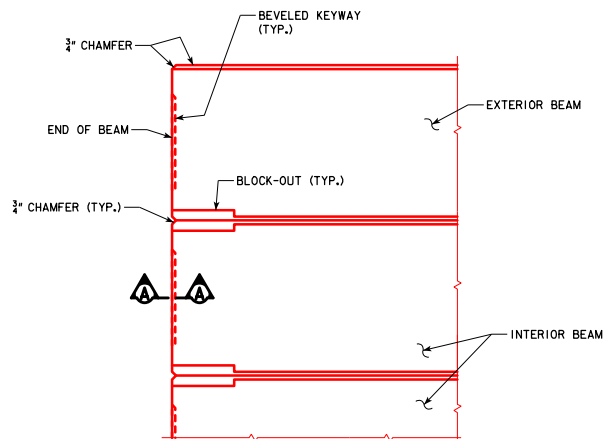
PARTIAL PLAN (0° SKEW)
