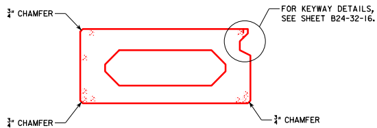
EXTERIOR BEAM
