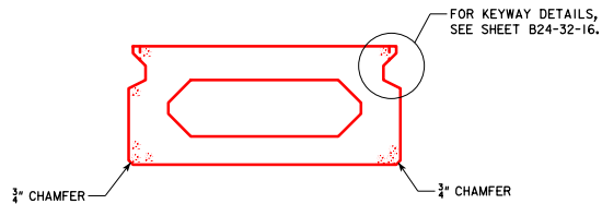
INTERIOR BEAM
