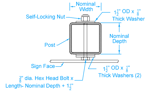
SHIM ATTACHMENT DETAIL FOR PSST POST
