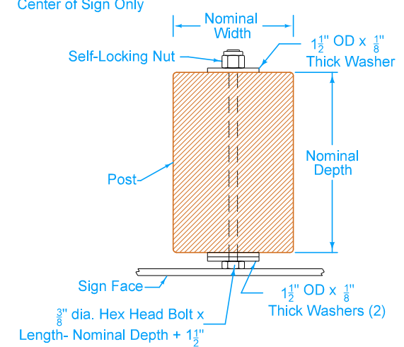
SHIM ATTACHMENT DETAIL FOR WOOD POST
