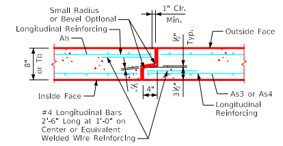
Tongue and Groove Joint Detail
