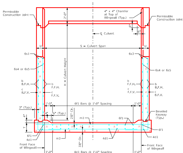
Typical Cross Section - thru Headwall
