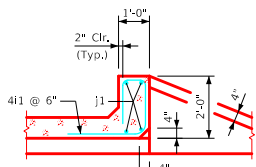
Section thru Parapet
