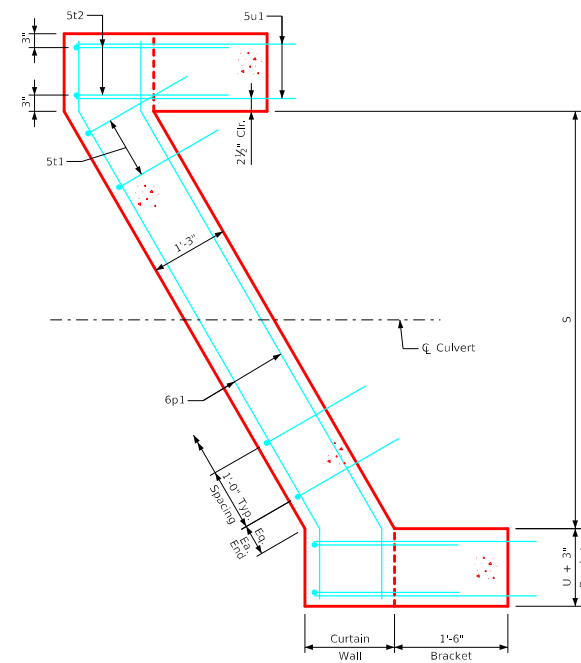
Curtain Wall Detail - Plan View
