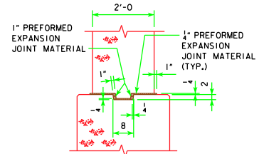
KEYED NOTCH DETAIL
