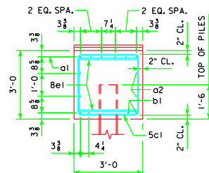
VIEW A-A FOR 7, 8, 9, 10, 11 & 12 PILE BENTS
