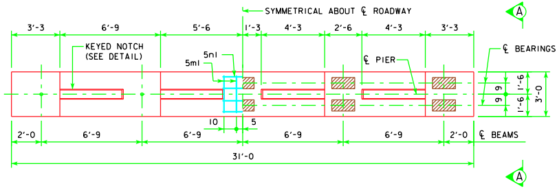
TYPICAL PLAN
