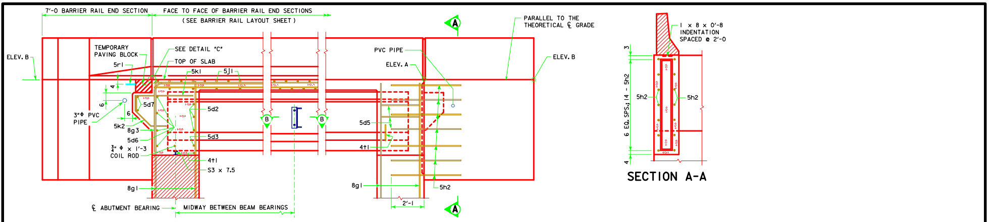
PART LONGITUDINAL SECTION NEAR GUTTER (FOR DETAILS OF INTERMEDIATE DIAPHRAGM SEE SHEET H30S1-30-12)
