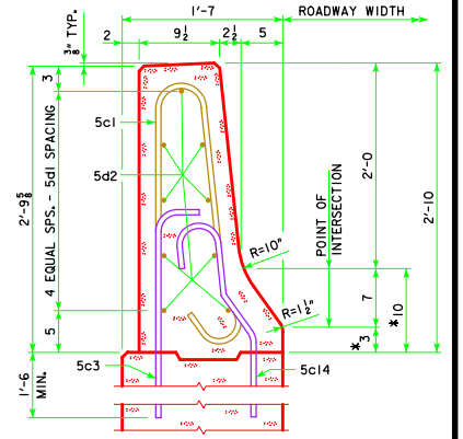
PART SECTION A-A
