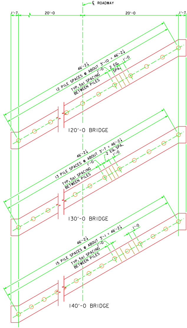
PILE PLAN - 30° SKEW WOOD PILING
