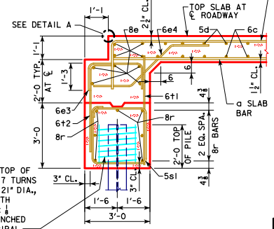
SECTION NORMAL TO ABUTMENT AT GUTTERLINE (BRIDGE LENGTHS 70'-110')
