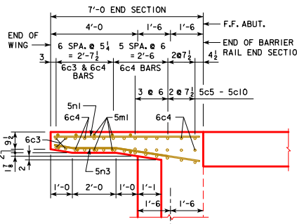
PART PLAN 0° SKEW (RAILING NOT SHOWN)
