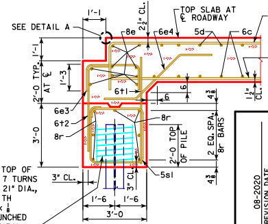
SECTION NORMAL TO ABUTMENT AT GUTTERLINE (BRIDGE LENGTHS 120'-150')
