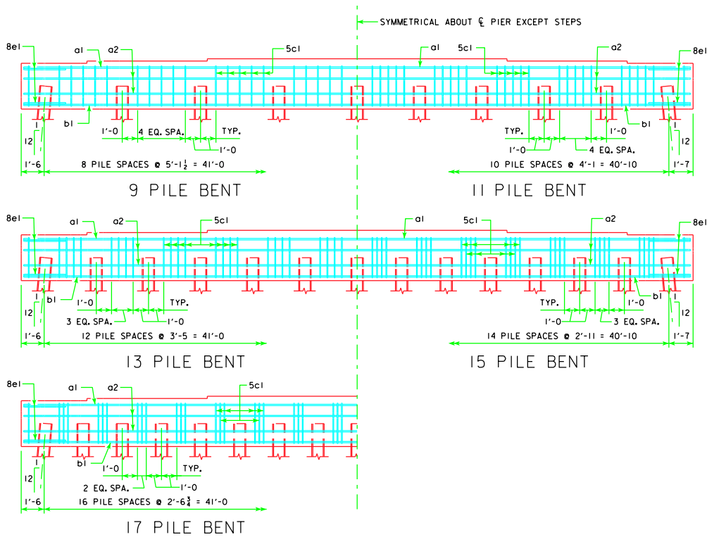
TYPICAL PLAN
