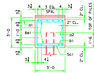
VIEW A-A FOR 9, 11, 13, 15 & 17 PILE BENTS
