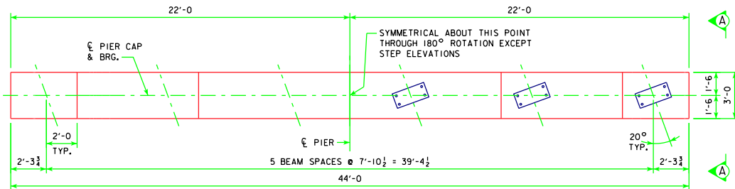
TYPICAL PLAN
