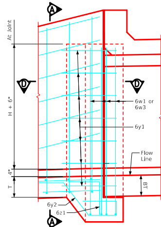
Part Elev. - Junction Bell Jt.
