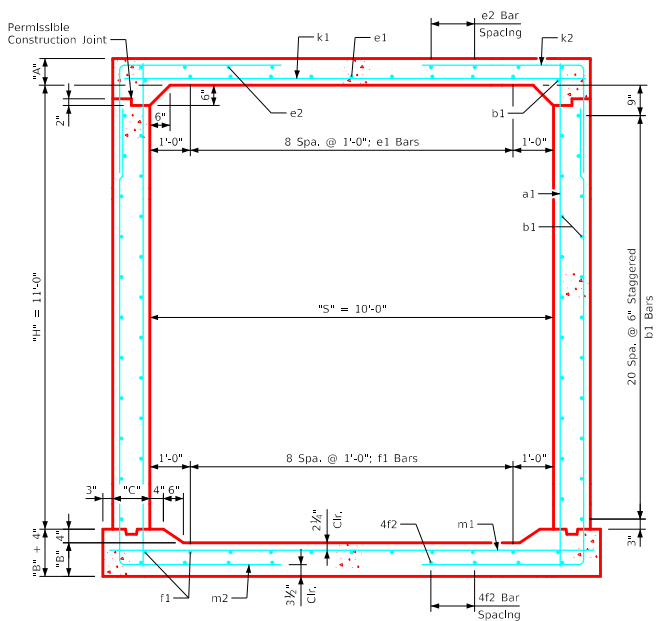
10' x 11' Barrel Section
