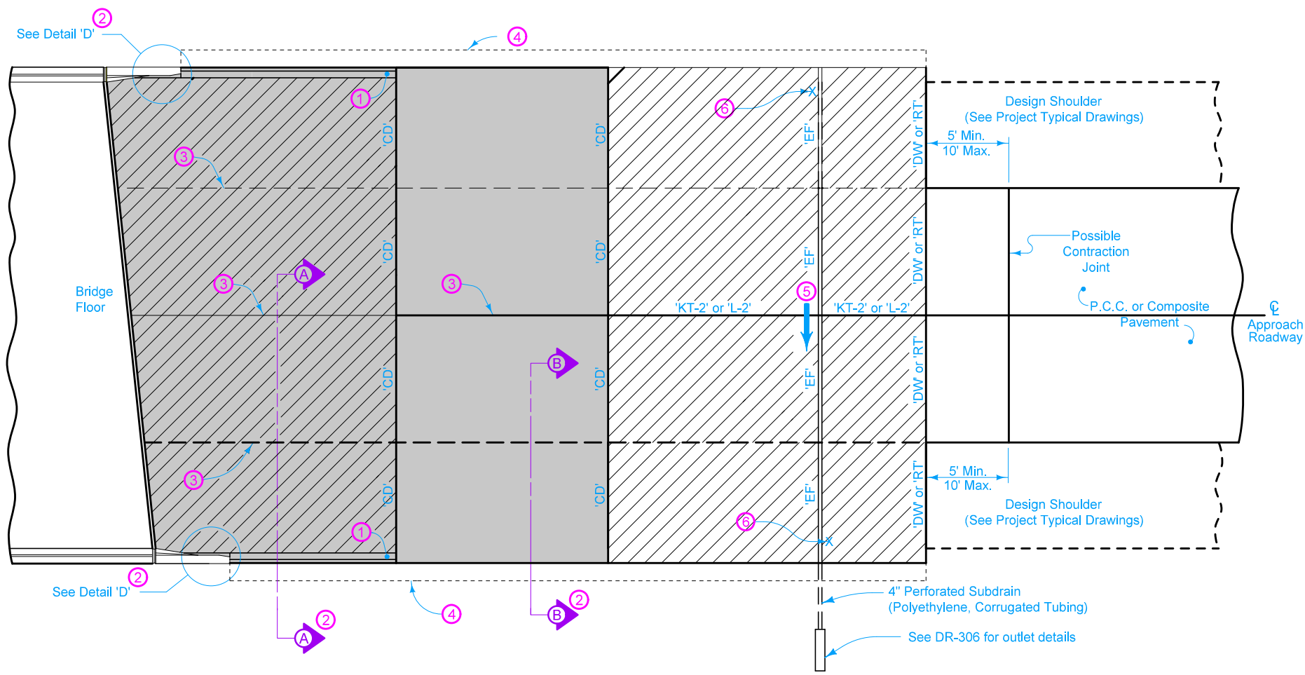
PLAN VIEW
